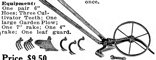
No. 11 Double and Single Wheel Equipment
